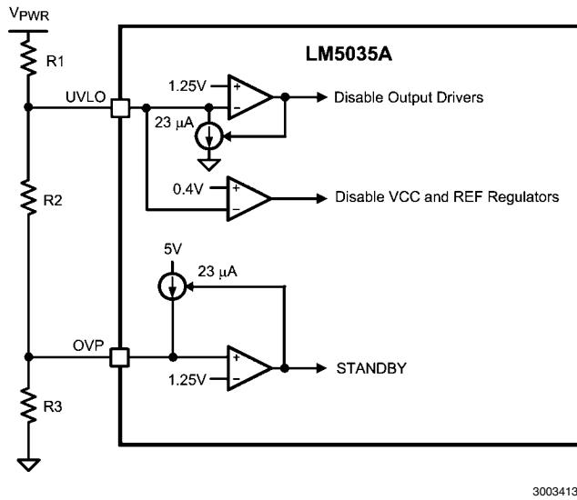
FIGURE 12. UVLO/OVP Divider
